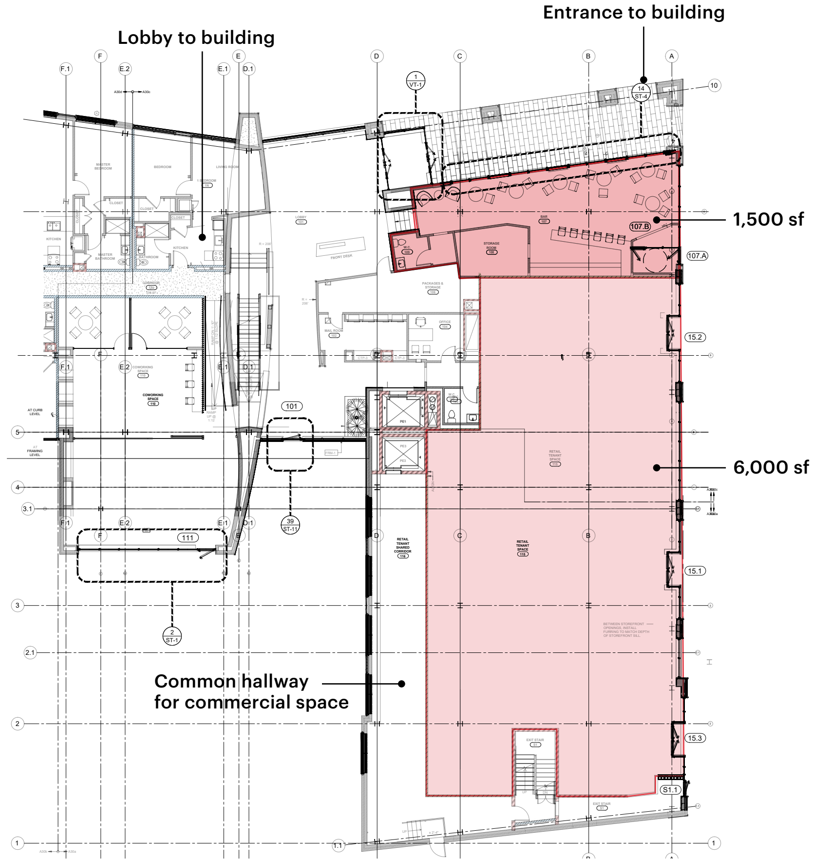
A 1ST FLOOR PLAN ARCH REF: A/A13
